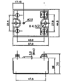
Mechanical Drawing
