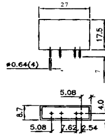
Mechanical Drawing
