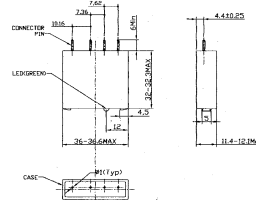
Mechanical Drawing
