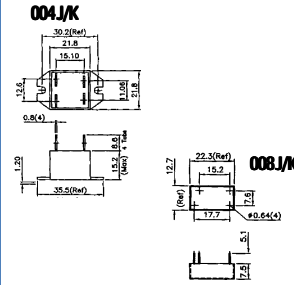
Mechanical Drawing
