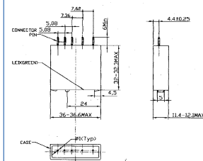
Mechanical Drawing
