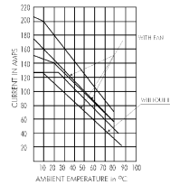
Derating Curve
