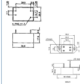
Mechanical Drawing
