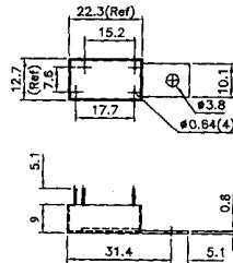
Mechanical Drawing
