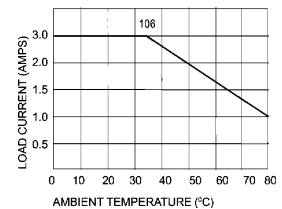
Derating Curve
