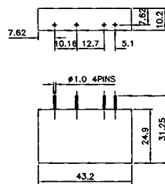
Mechanical Drawing
