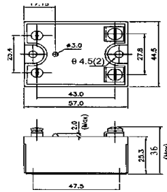
Mechanical Drawing
