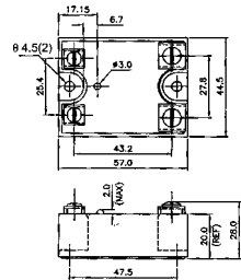
Mechanical Drawing
