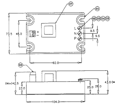
Mechanical Drawing
