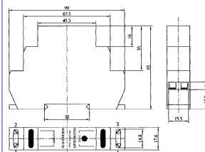
Mechanical Drawing
